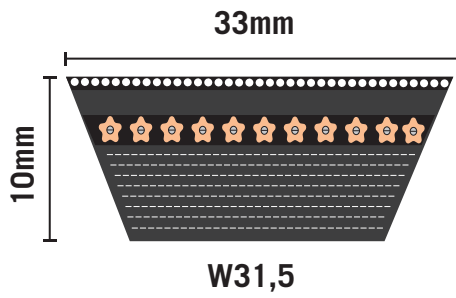
Standard Belt Range
